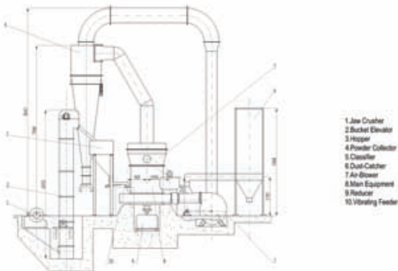
YGM130 High-pressure Suspension Mill Diagram of the Equipment
